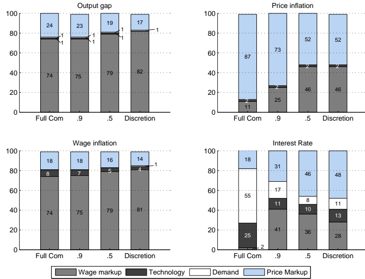
Figure 6: Variance decomposition
