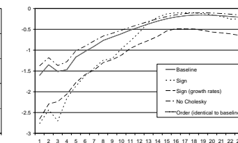
C) Restrictions
