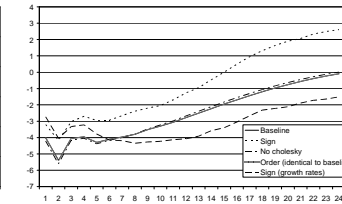
C) Restrictions
