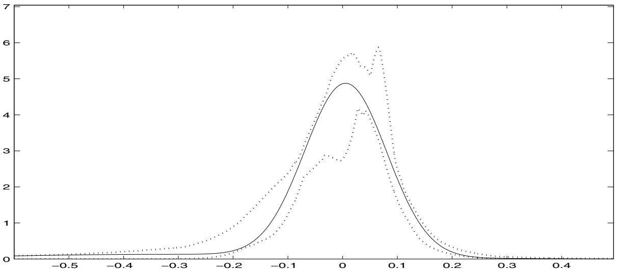
Figure 10: Implied distribution extracted by DLN at September 24, 2001, together with the corresponding confidence band
