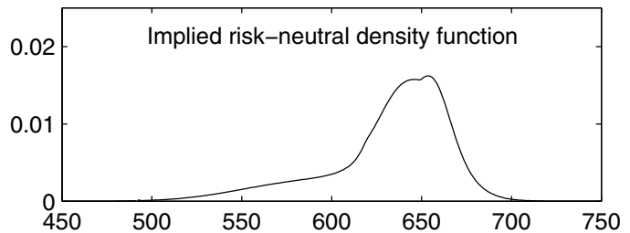
Figure 4.2: Steps in the smoothed implied volatility smile method
