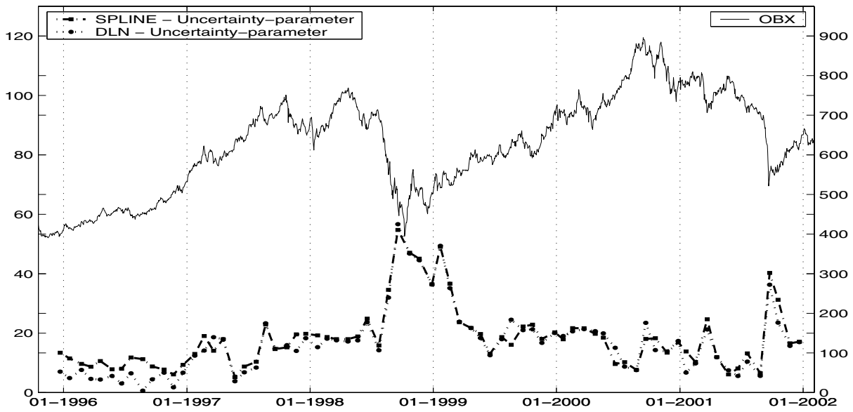
Figure 21: Uncertainty-parameter vs OBX index
