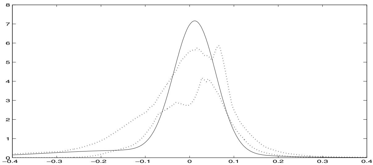
Figure 16: Confidence band for DLN at September 24, and implied distribution extracted at October 19
