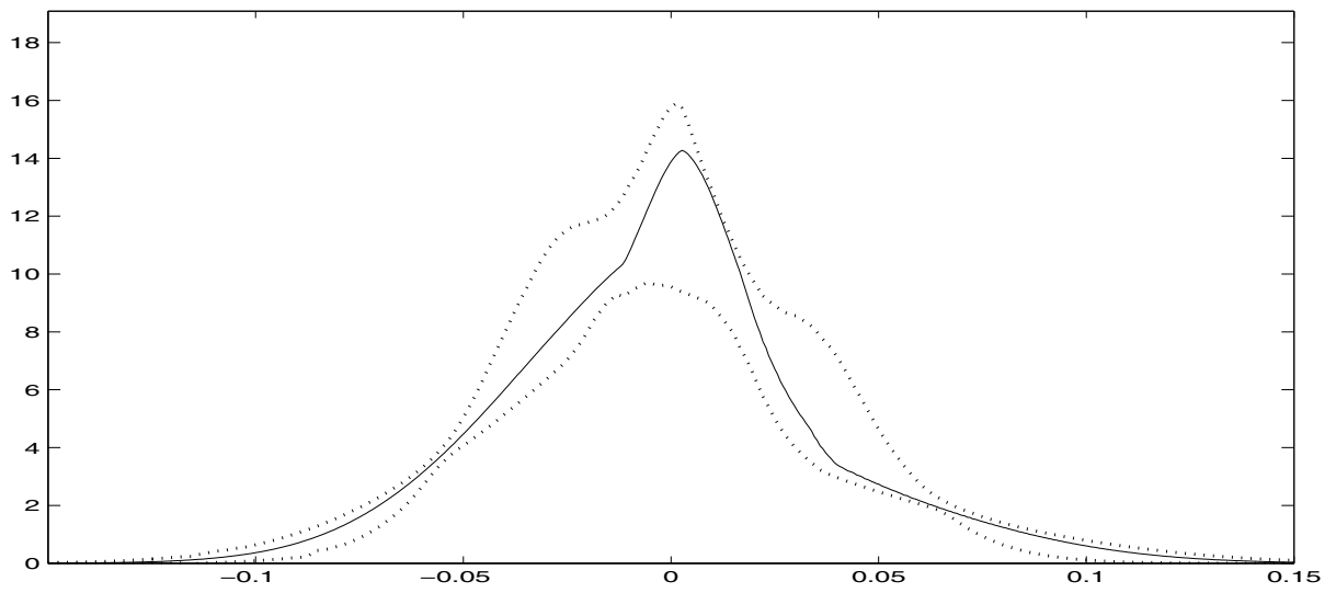
Figure 7: Implied distribution extracted by SPLINE at August 27, 2001, together with the corresponding confidence band
