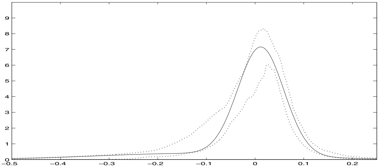
Figure 12: Implied distribution extracted by DLN at October 19, 2001, together with the corresponding confidence band
