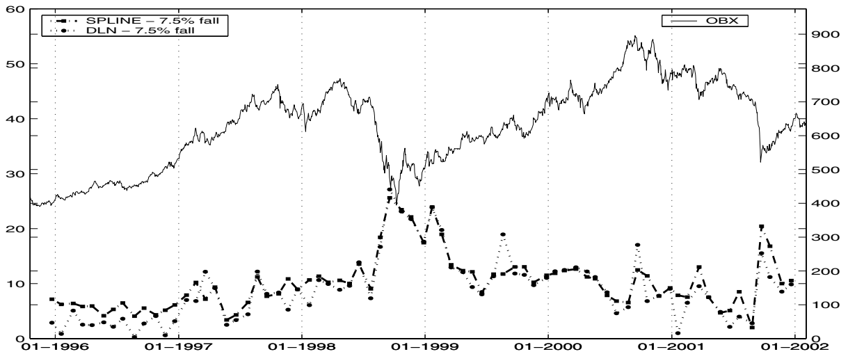
Figure 5.9: Implied risk-neutral probability of a fall in the OBX index of 7.5 percent or more relative to the futures price the next four weeks vs OBX index (equal to Figure 20 in Appendix C)
