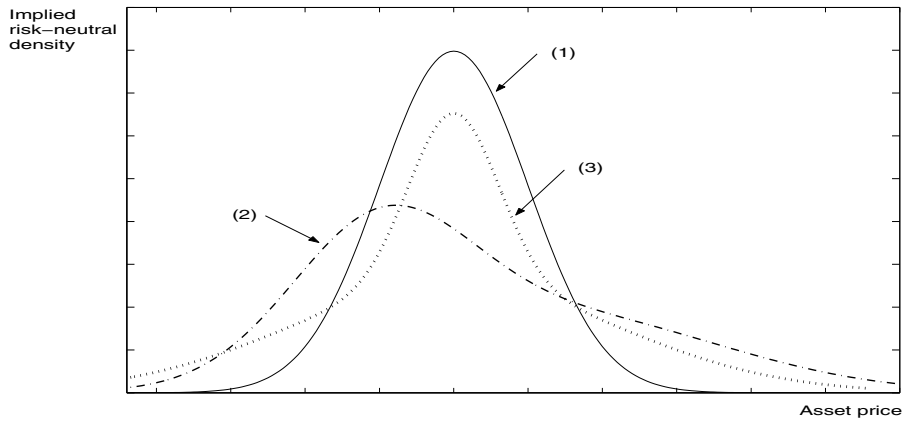
Figure 1.1: Examples of implied risk-neutral density functions
