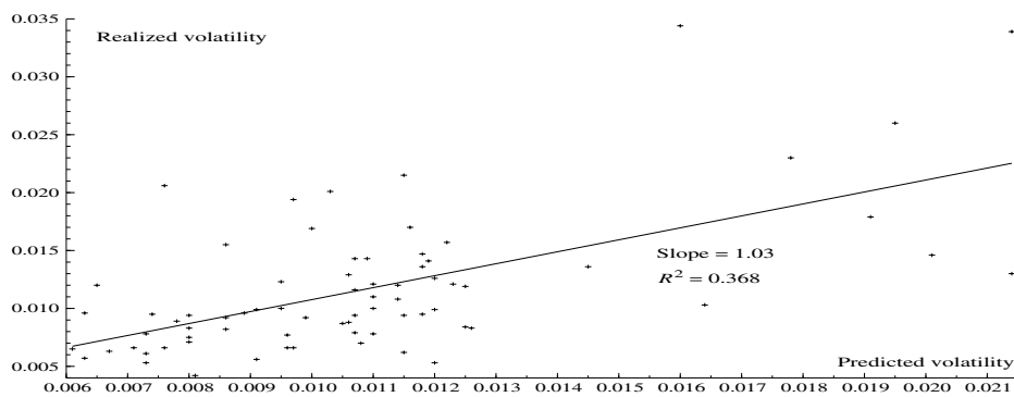
Figure 25: Scatter plots of realized volatility versus predicted volatility (using SLN)
