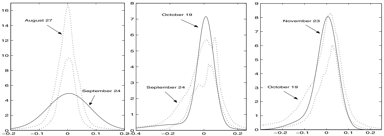
Figure 5.8: Confidence bands (dotted lines) and implied distributions (solid lines) extracted the following month
