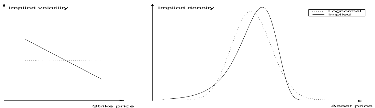
Figure 2.3: A skewed volatility smile and the corresponding implied distribution
