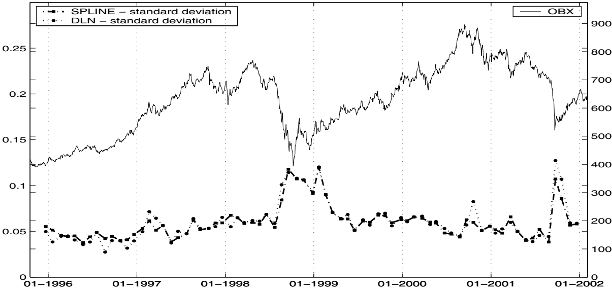
Figure 19: Implied standard deviation vs OBX index
