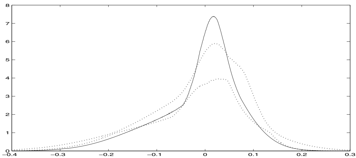
Figure 15: Confidence band for SPLINE at September 24, and implied distribution extracted at October 19
