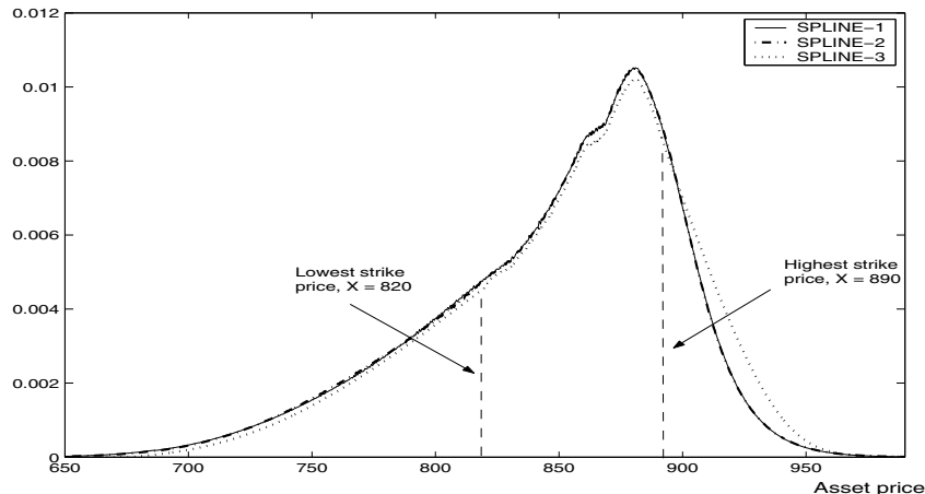
Figure 5.4: Implied risk-neutral density functions extracted by the different SPLINE methodologies at September 22, 2000
