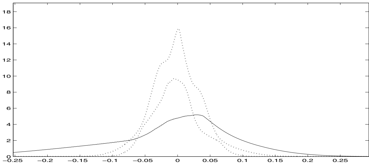
Figure 13: Confidence band for SPLINE at August 27, and implied distribution extracted at September 24
