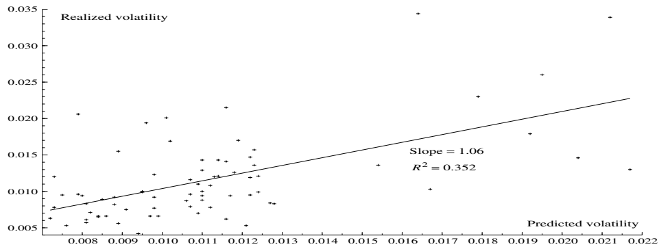
Figure 23: Scatter plots of realized volatility versus predicted volatility (using SPLINE)
