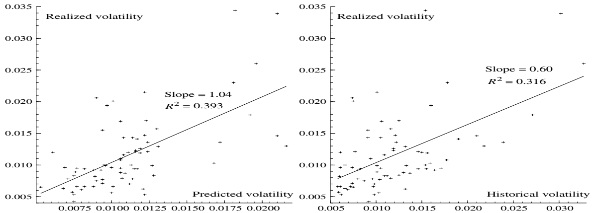
Figure 5.12: Scatter plots of realized volatility versus predicted volatility (using DLN) and realized volatility versus historical volatility (left panel equal to Figure 24 in Appendix C)
