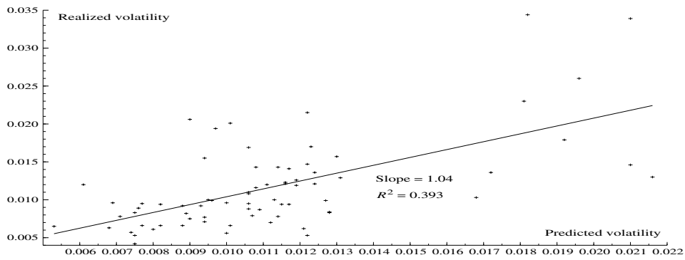
Figure 24: Scatter plots of realized volatility versus predicted volatility (using DLN, equal to Figure 5.12 in Section 5.5.2)
