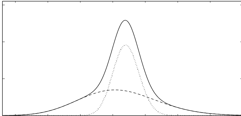
Figure 4.1: Example of a double lognormal distribution
