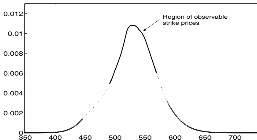
Figure 4.5: Connecting lognormal distributions at the tails of the implied risk-neutral density function
