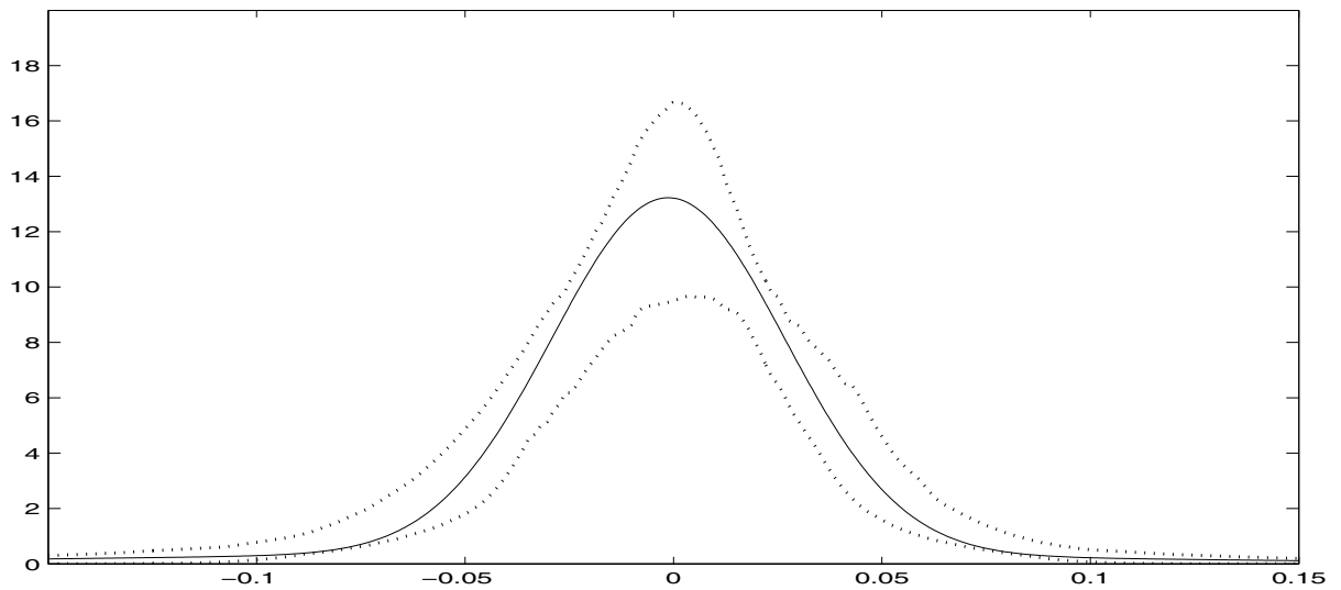
Figure 8: Implied distribution extracted by DLN at August 27, 2001, together with the corresponding confidence band
