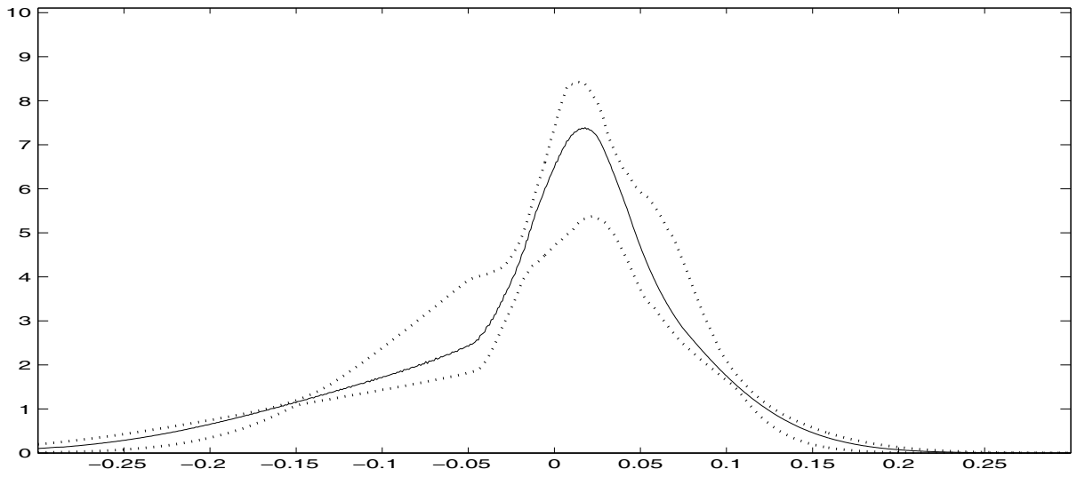
Figure 11: Implied distribution extracted by SPLINE at October 19, 2001, together with the corresponding confidence band
