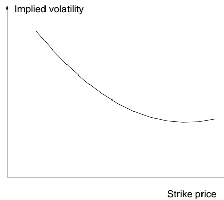
Figure 2.2: A typical volatility smile for an equity option
