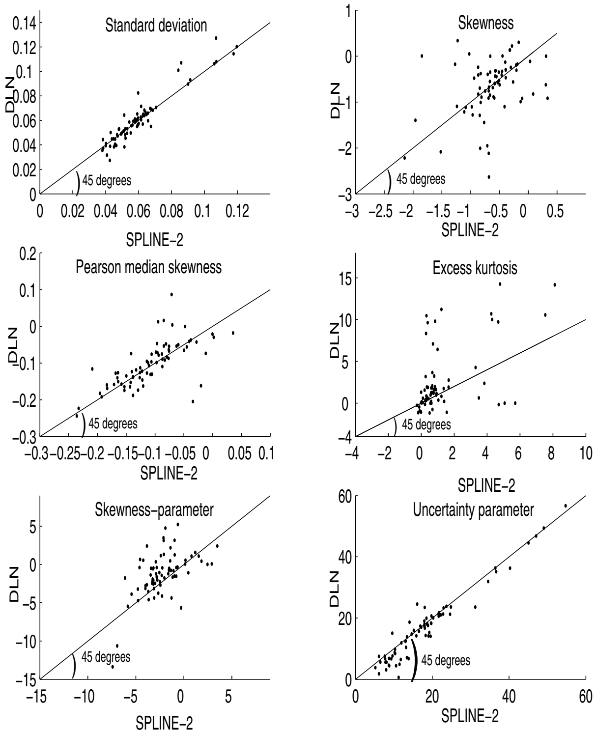
Figure 6: Scatter plot of SPLINE-2 and DLN
