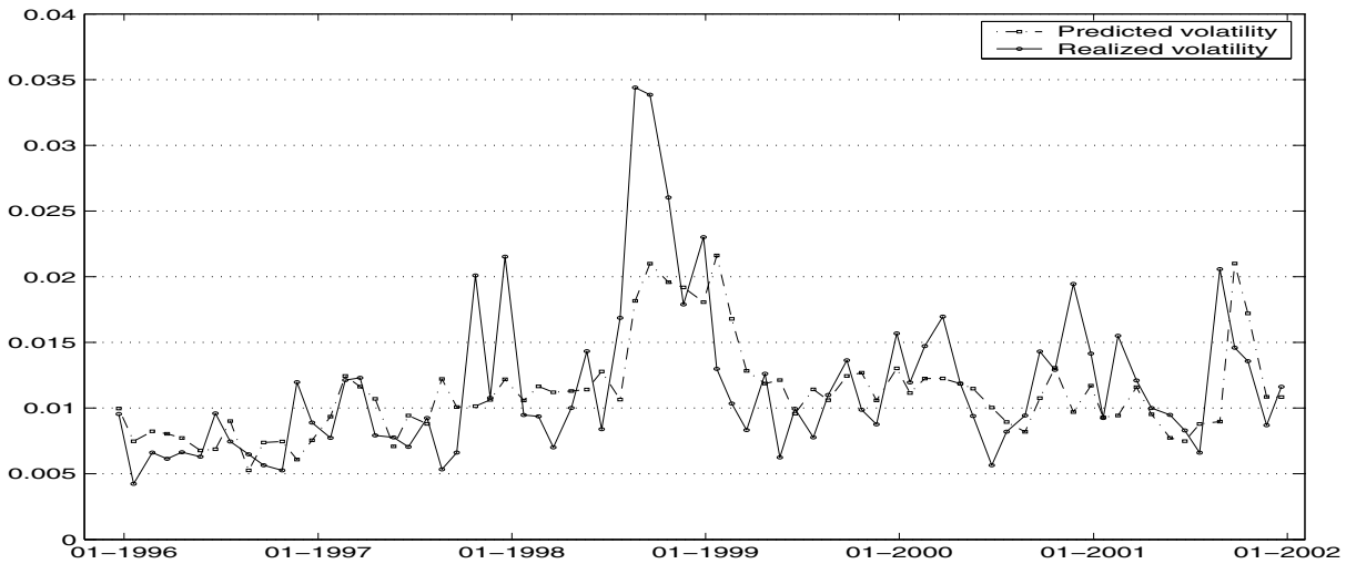
Figure 5.11: Predicted volatility (DLN) and realized volatility
