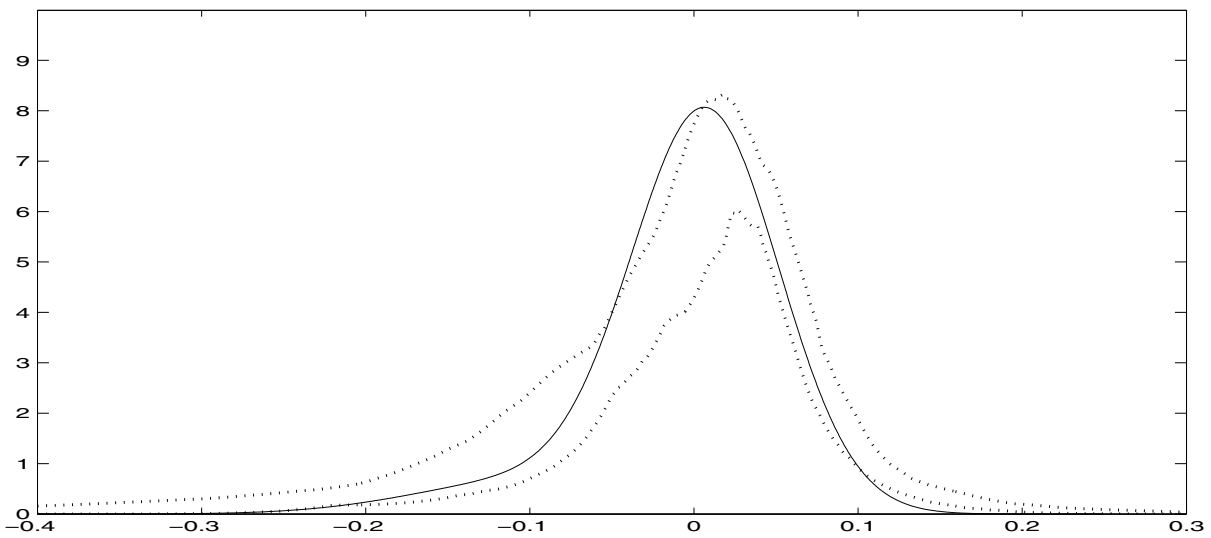
Figure 18: Confidence band for DLN at October 19, and implied distribution extracted at November 23
