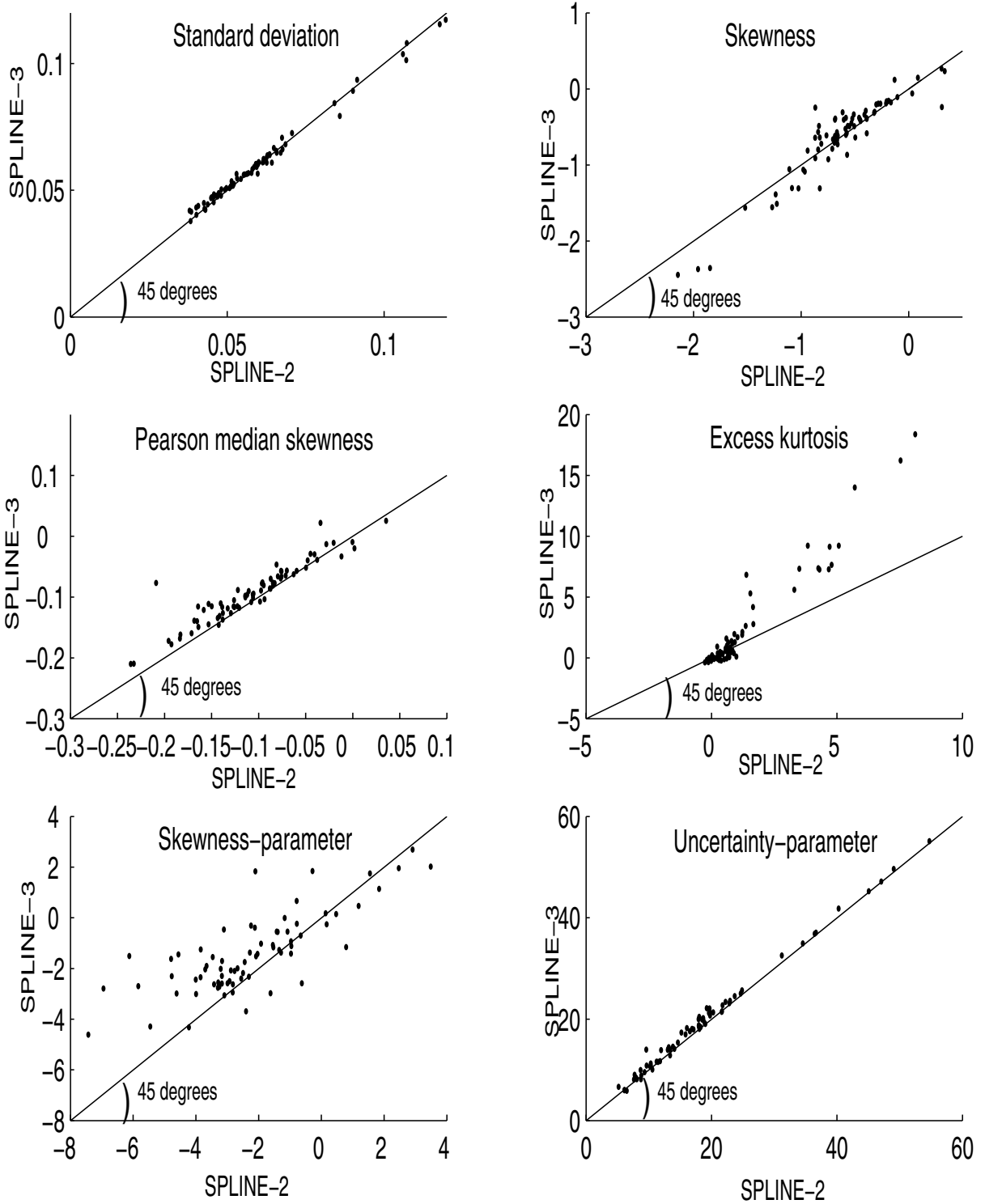
Figure 3: Scatter plot of SPLINE-2 and SPLINE-3
