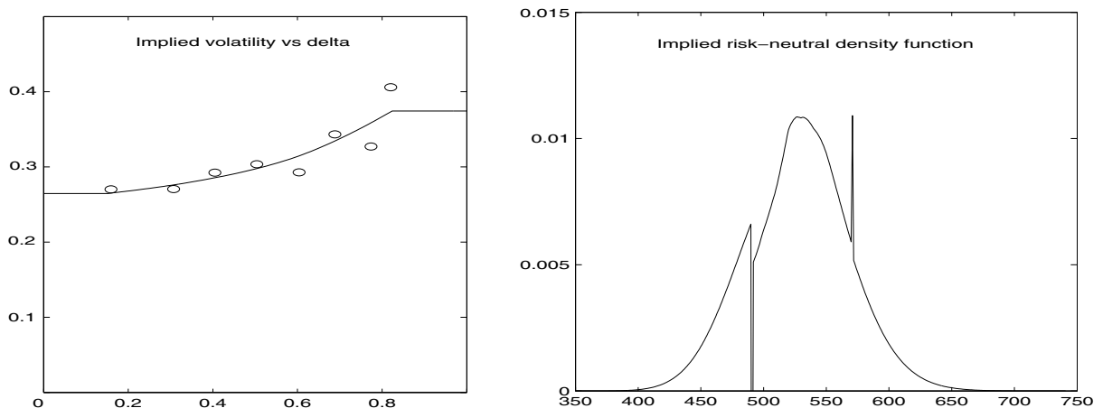
Figure 4.4: Implications of a too abrupt change in the implied volatility curve
