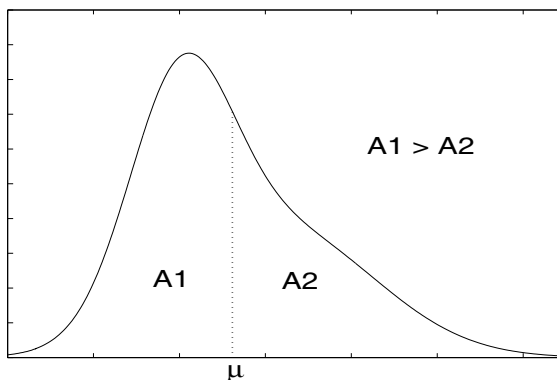
Figure 4.6: A positively skewed distribution
