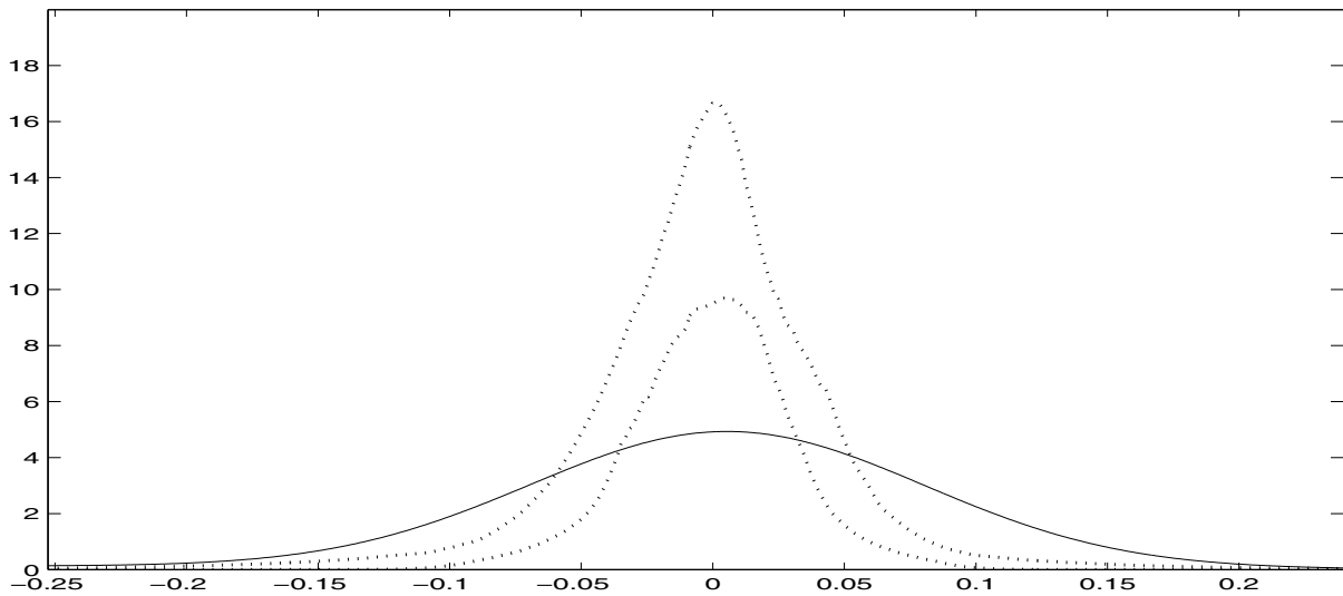
Figure 14: Confidence band for DLN at August 27, and implied distribution extracted at September 24
