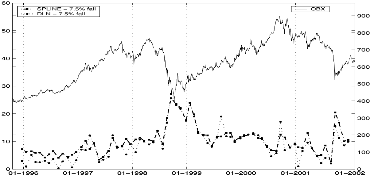
Figure 20: Implied risk-neutral probability of a fall in the OBX index of 7.5 percent or more relative to the futures price the next four weeks vs OBX index (equal to Figure 5.9 in Section 5.5.1)
