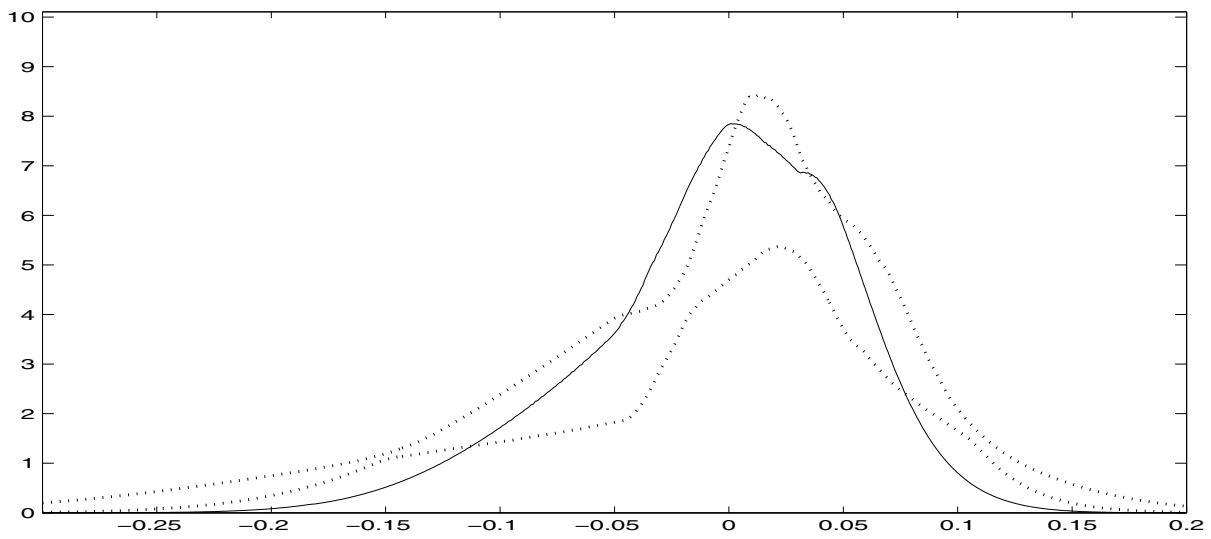
Figure 17: Confidence band for SPLINE at October 19, and implied distribution extracted at November 23
