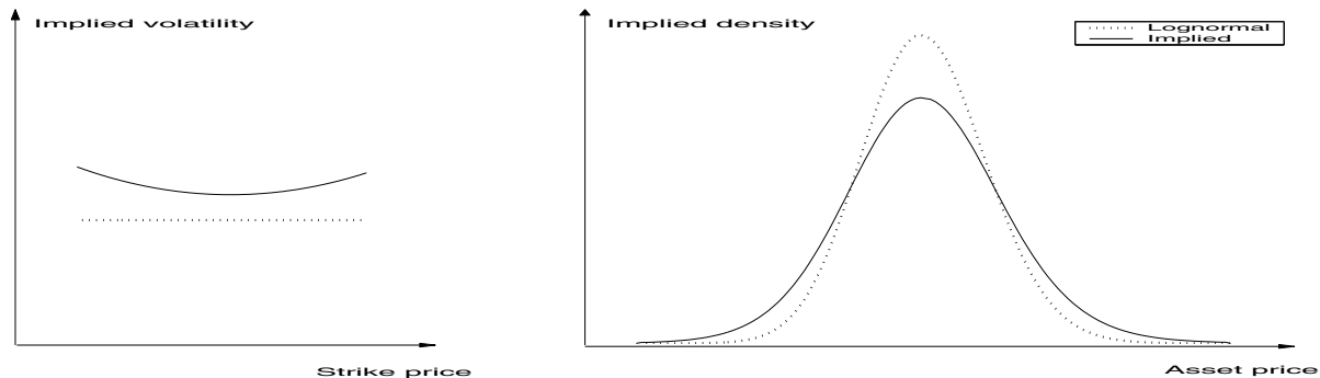
Figure 2.4: A convex volatility smile and the corresponding implied distribution
