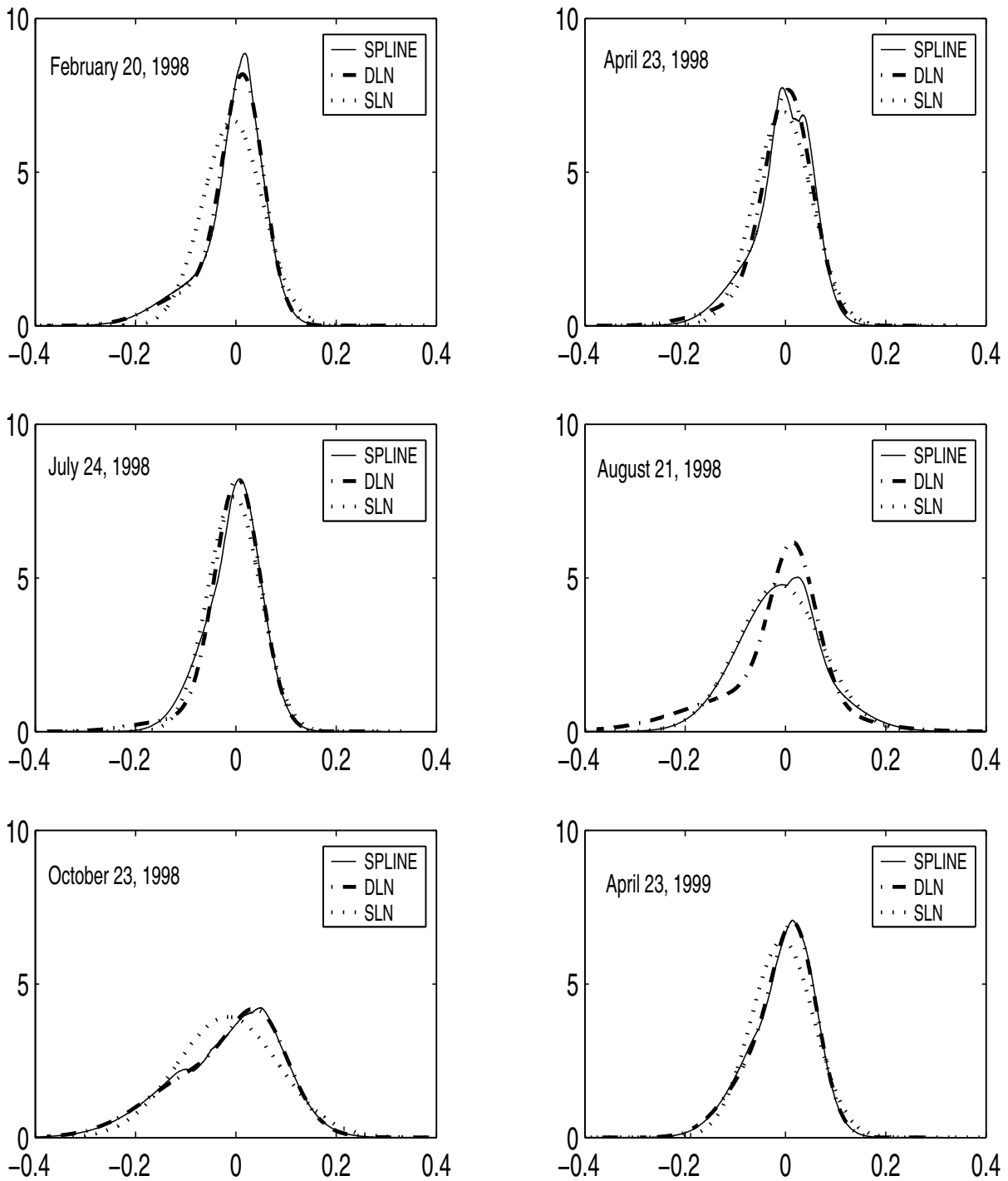
Figure 5.3: Implied (logarithmic) return distributions extracted around the Russian crisis
