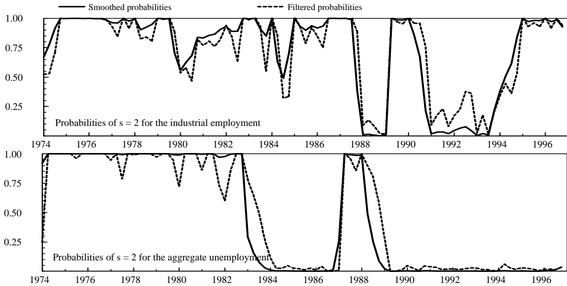
Figure 6: The filtered and smoothed probabilities of industrial employment and aggregate unemployment being in state 2: the expansion phase.
