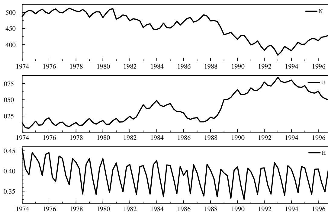
Figure 1: Time series of the Y variables (in levels) over the sample period: 1974(1)–1996(4). Persons employed in manufacturing and construction in thousands ( N ), the aggregate unemployment rate ( U ) and average working hours in manufacturing and construction ( H ) in thousands.
