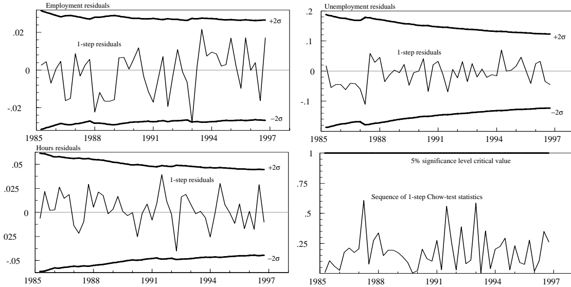
Figure 5: 1-step ahead residuals \pm 2 estimated standard errors based on the equations of employment, unemployment and hours. Also, a sequence of 1-step Chow tests scaled by their critical values at the 5% level of significance.
