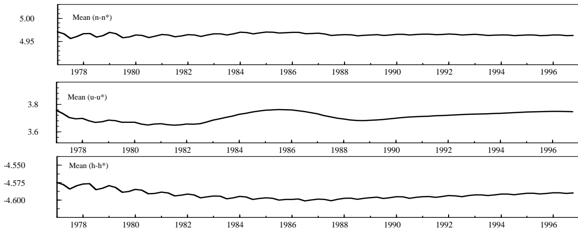
Figure 4: Recursive estimates of the means of n - n^* , u - u^* and of h - h^* over the period 1977(1)–1996(4). The initial estimates are based on observations from the period 1974(1)–1976(4).
