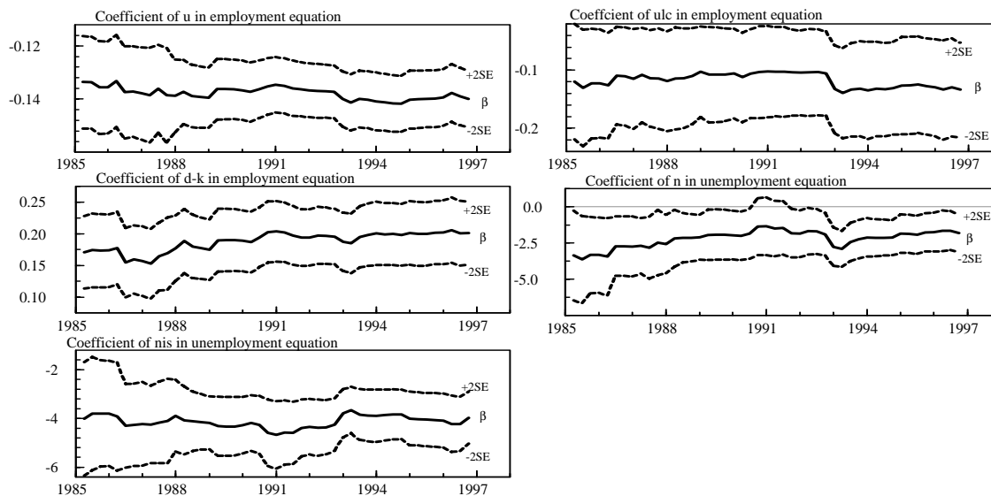
Figure 3: Recursive estimates of the cointegration vectors with \pm 2SE . Initial sample: 1974(1)–1984(4).
