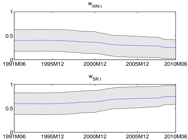
Figure 12: Combination weights for the S&P 500 forecasts
