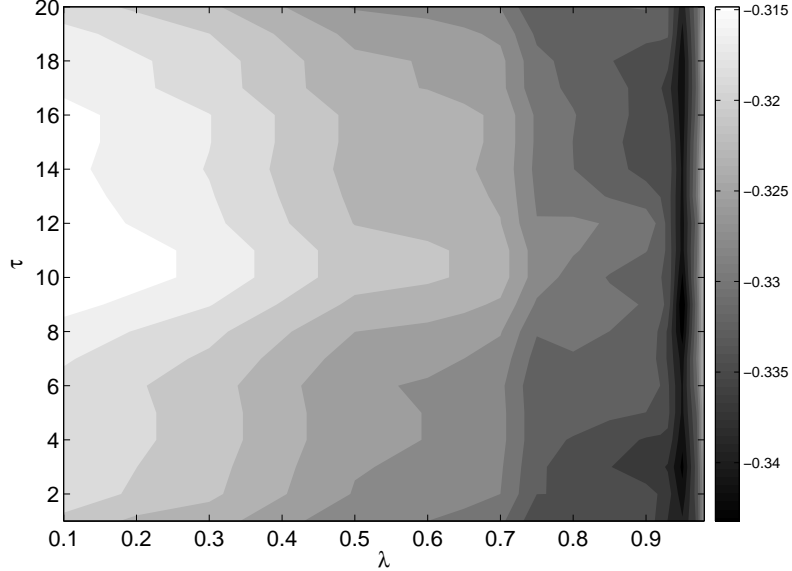
Figure 8: Optimal combination learning parameters
