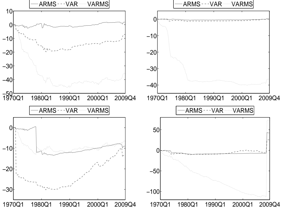
Figure 3: Cumulative Square Prediction Error and Log Score Differences
