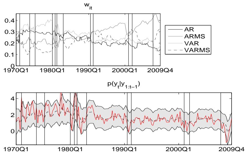
Figure 5: Combination forecasts with time-varying weights with learning
