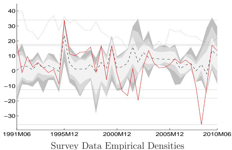
Figure 2: Livingston survey fan charts for the S&P 500
