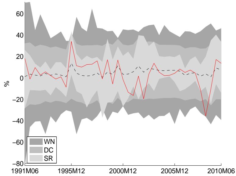
Figure 11: Prediction densities for S&P 500
