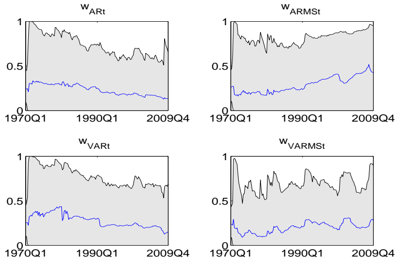
Figure 6: Time-varying weights without learning
