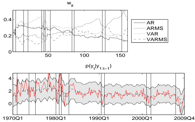
Figure 4: Combination forecasts with time-varying weights without learning
