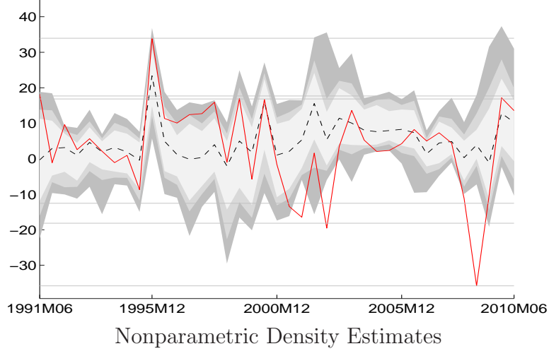
Figure 10: Livingston survey fan charts for the S&P500
