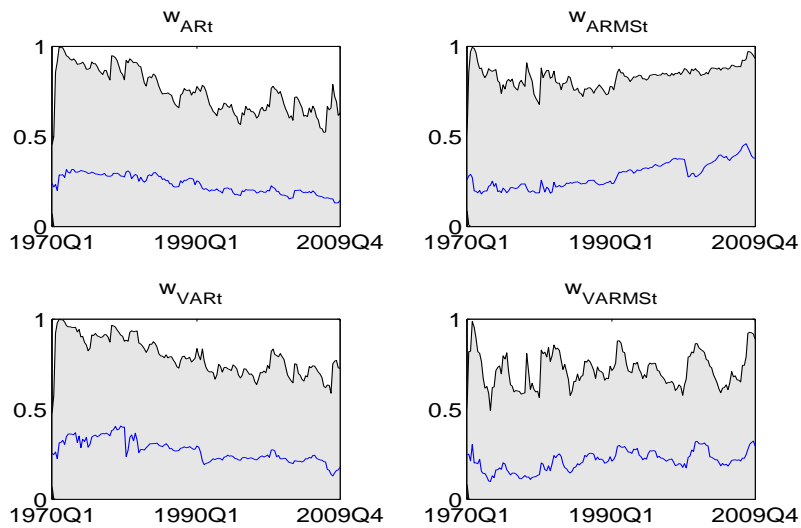
Figure 7: Time-varying weights with learning
